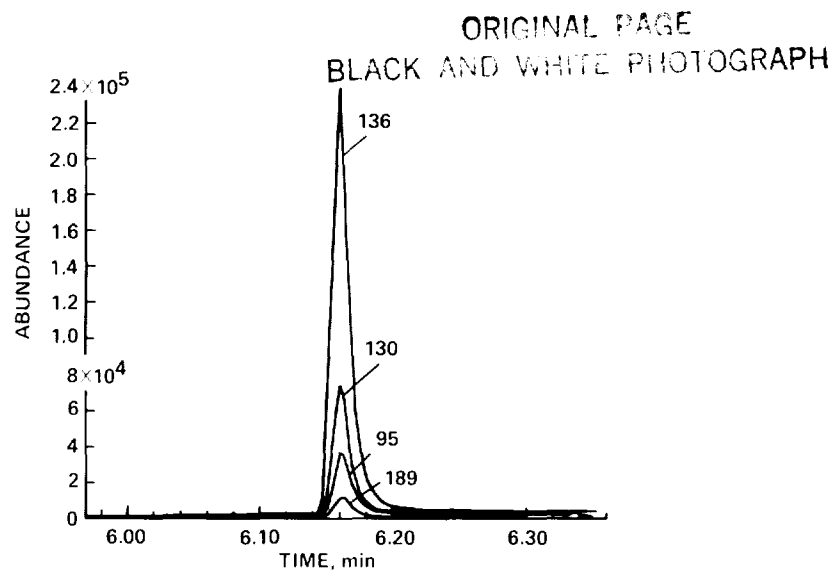
Fig. 5. Monitoring of masses 195 and 189, the molecular ions of the methyl ester of 6 C 13 IAA and plant IAA, and 136 and 130, the quinolinium ions of 6 C 13 IAA and plant IAA. Agreement of the ratio 195/189 and 136/130 is usually within 0.1% giving assurance that the compound being measured is, in fact, IAA.
